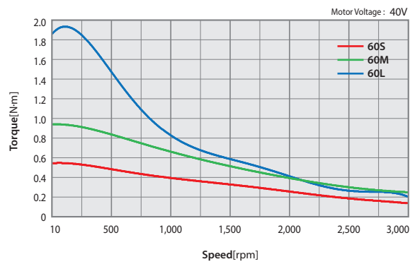
Ezi-STEP-MPB-60 series
